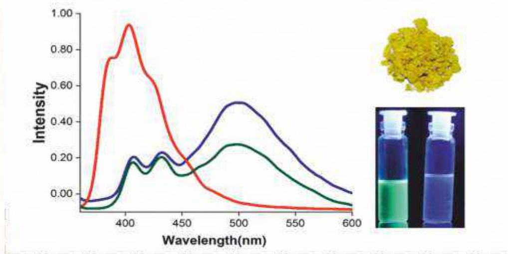
Overlaid fluorescence spectra of emissive organic materials
